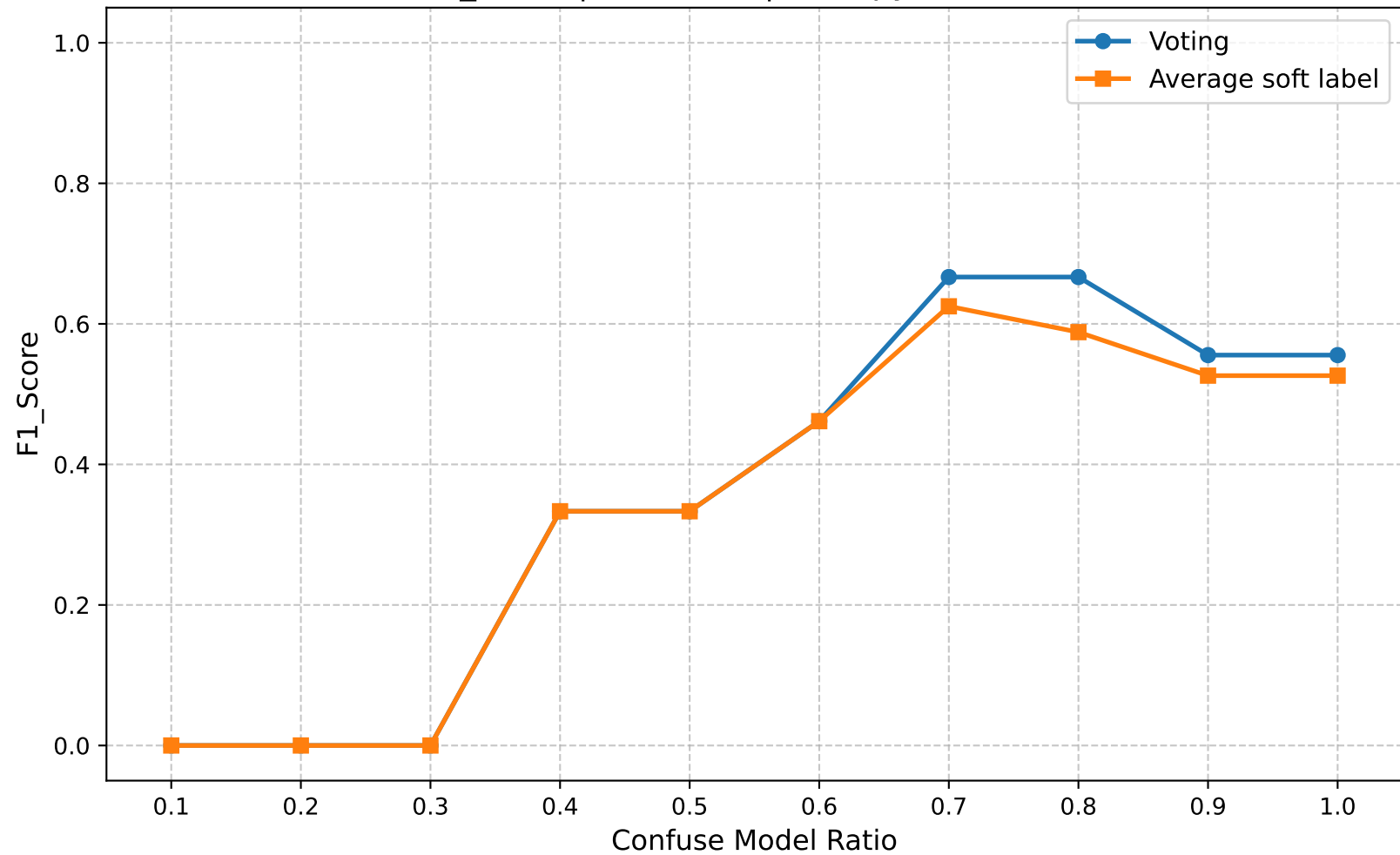
F1_Score | Round 10 | Entropy Ratio 0.15
