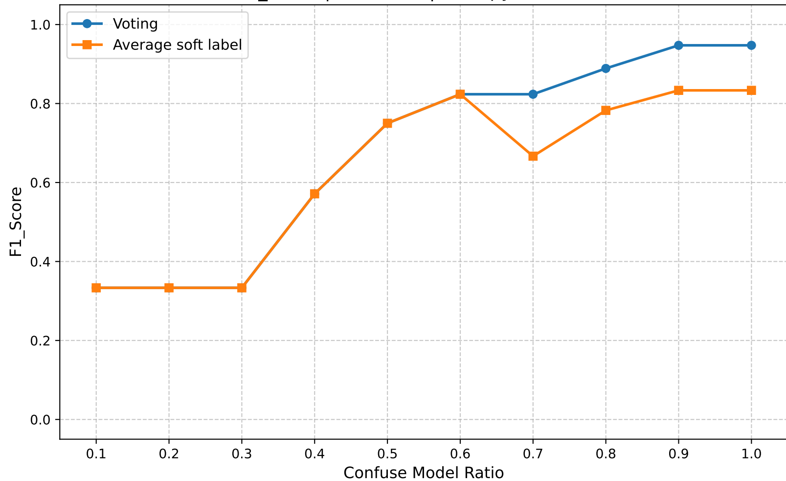
F1_Score | Round 10 | Entropy Ratio 0.30
