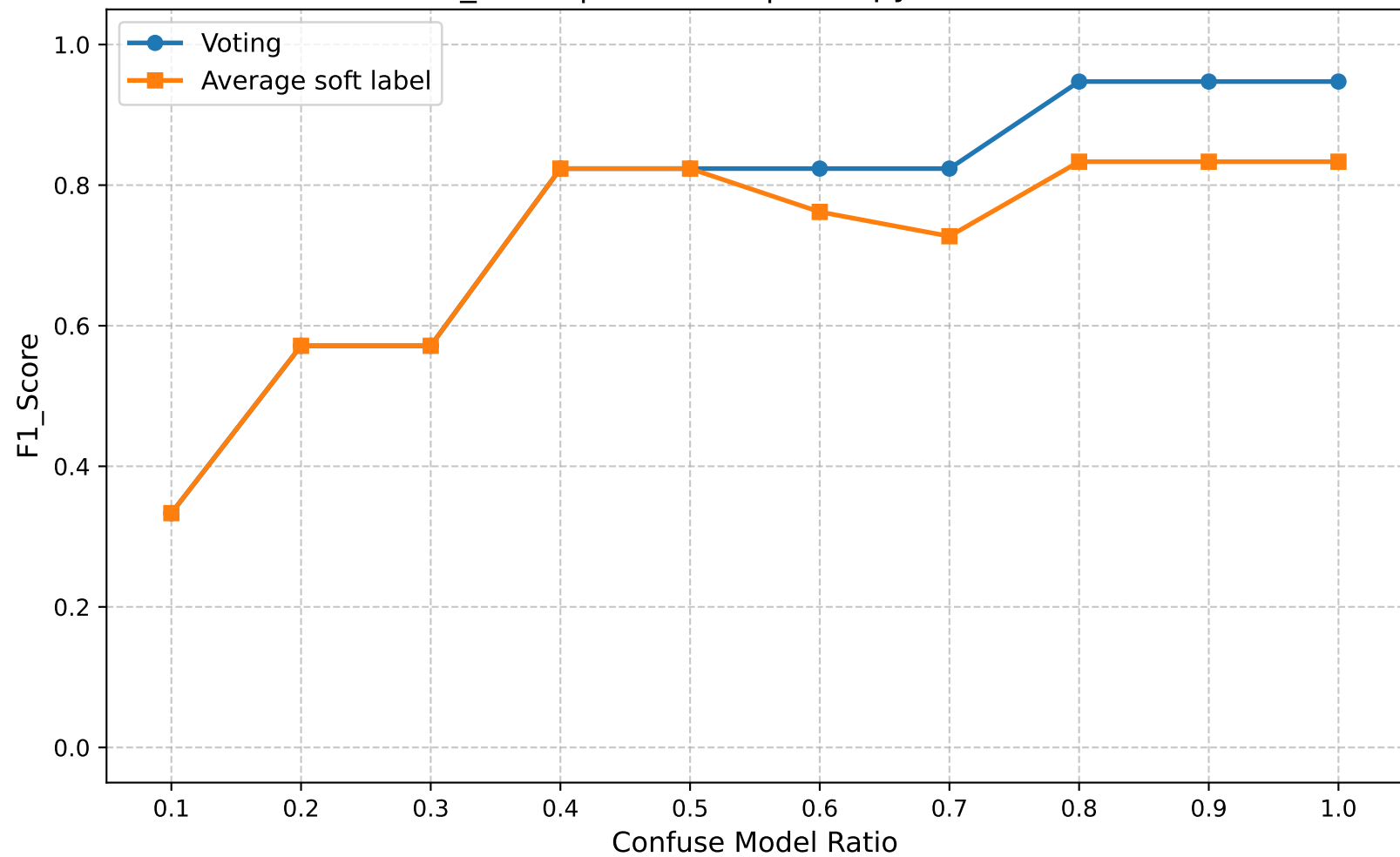
F1_Score | Round 10 | Entropy Ratio 0.35
