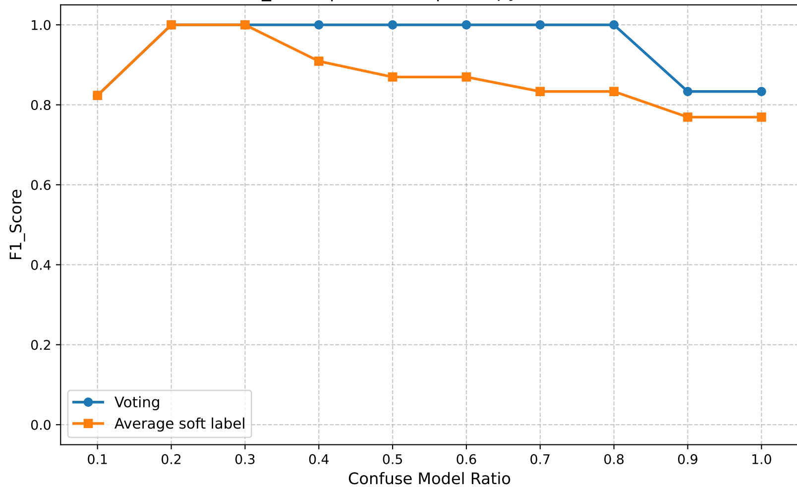
F1_Score | Round 10 | Entropy Ratio 0.60
