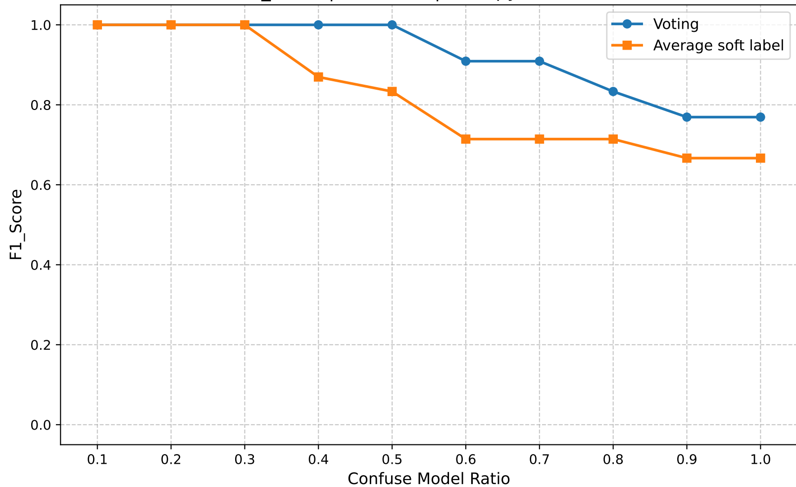
F1_Score | Round 10 | Entropy Ratio 0.75
