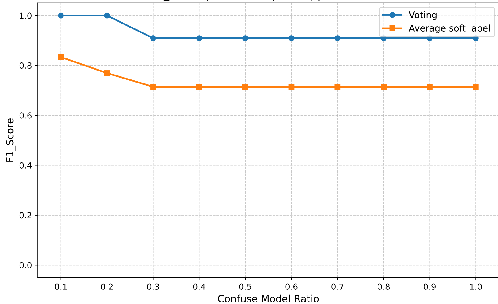
F1_Score | Round 10 | Entropy Ratio 0.95
