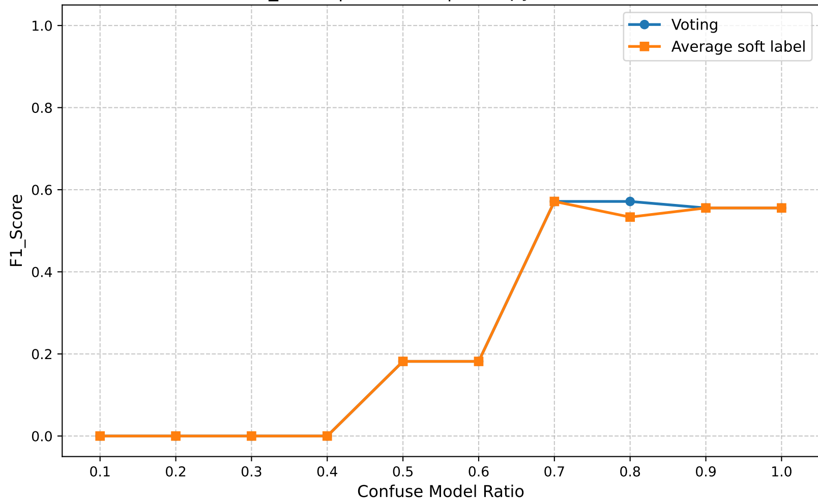
F1_Score | Round 15 | Entropy Ratio 0.15
