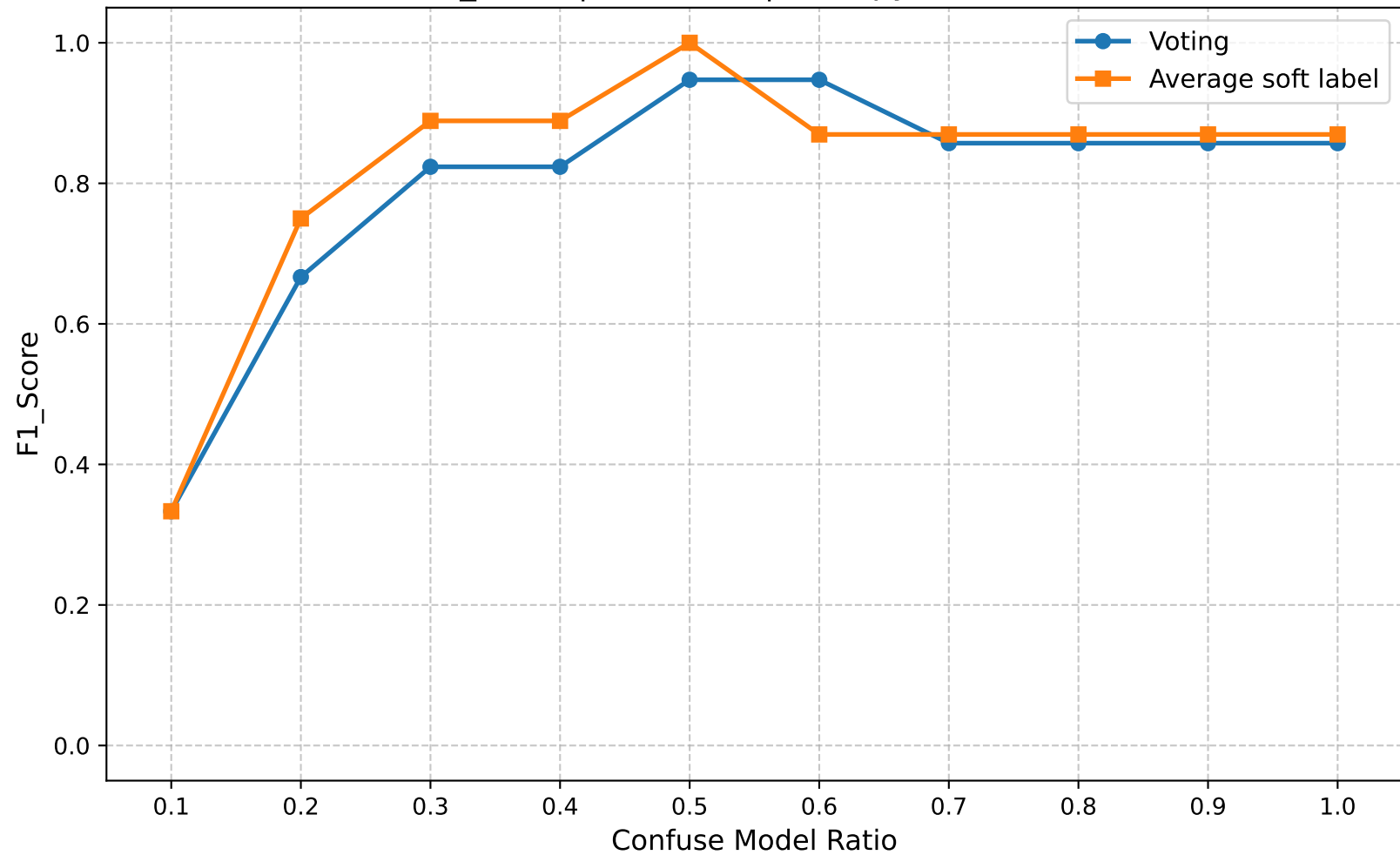
F1_Score | Round 15 | Entropy Ratio 0.45
