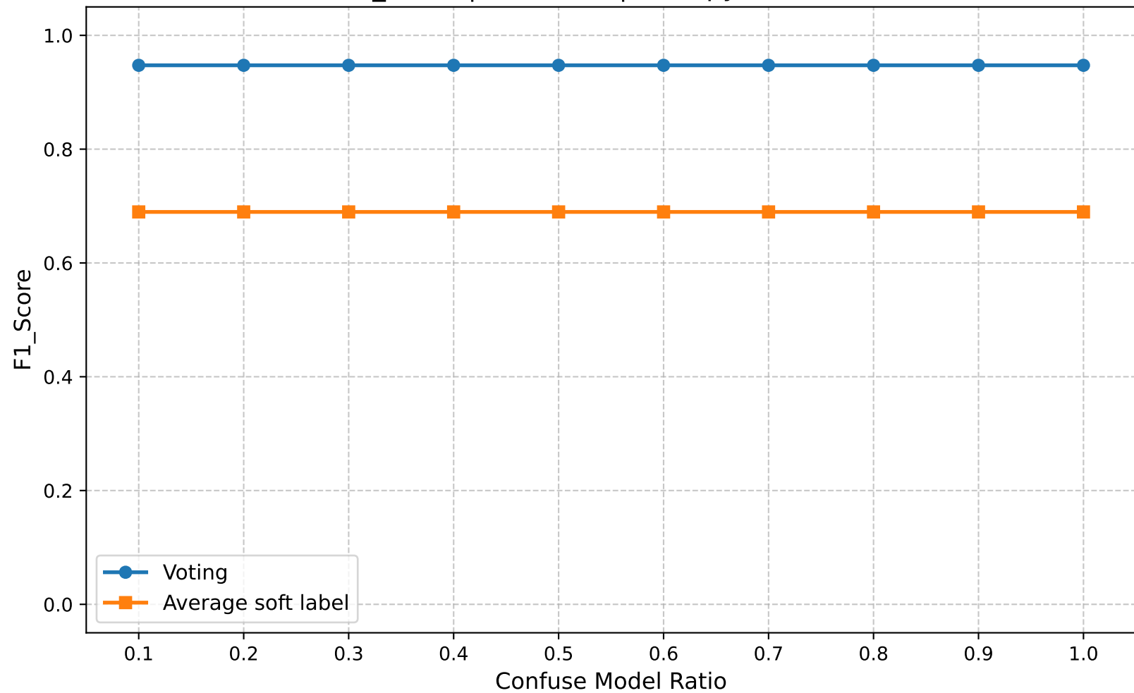
F1_Score | Round 15 | Entropy Ratio 1.00
