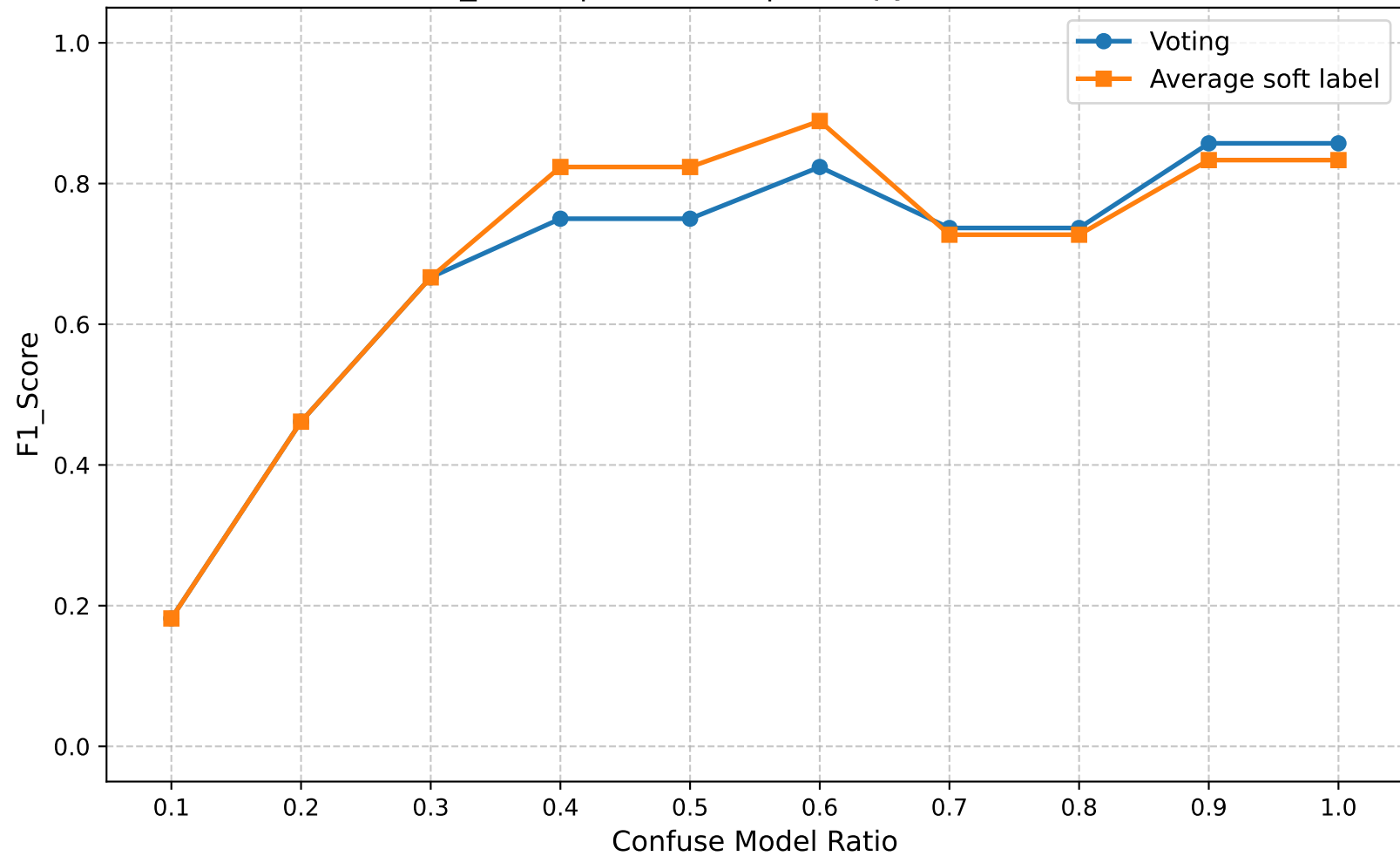
F1_Score | Round 20 | Entropy Ratio 0.35
