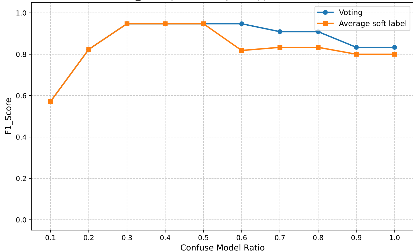
F1_Score | Round 20 | Entropy Ratio 0.50
