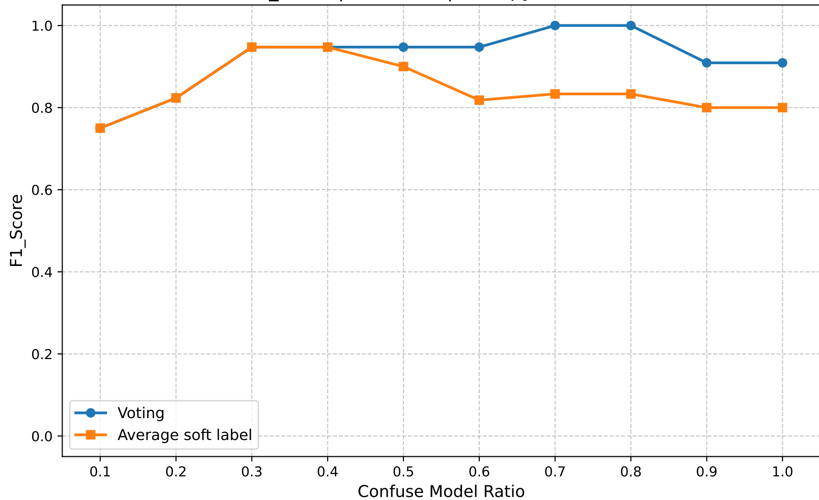
F1_Score | Round 20 | Entropy Ratio 0.55
