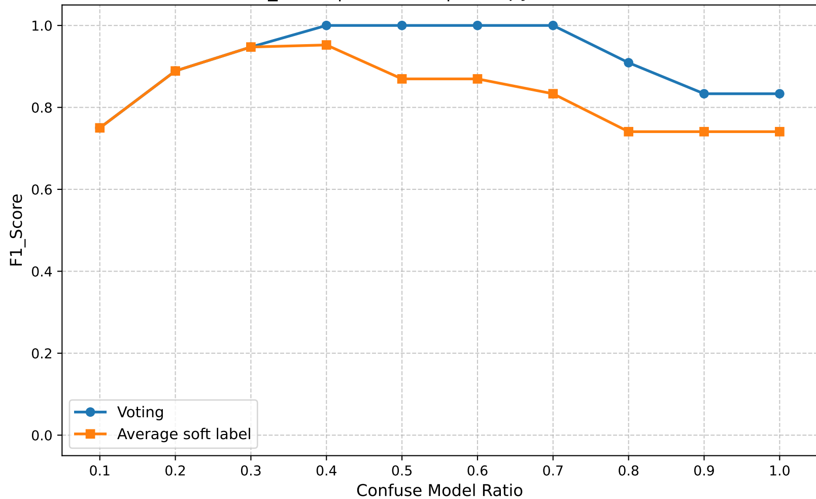
F1_Score | Round 20 | Entropy Ratio 0.60
