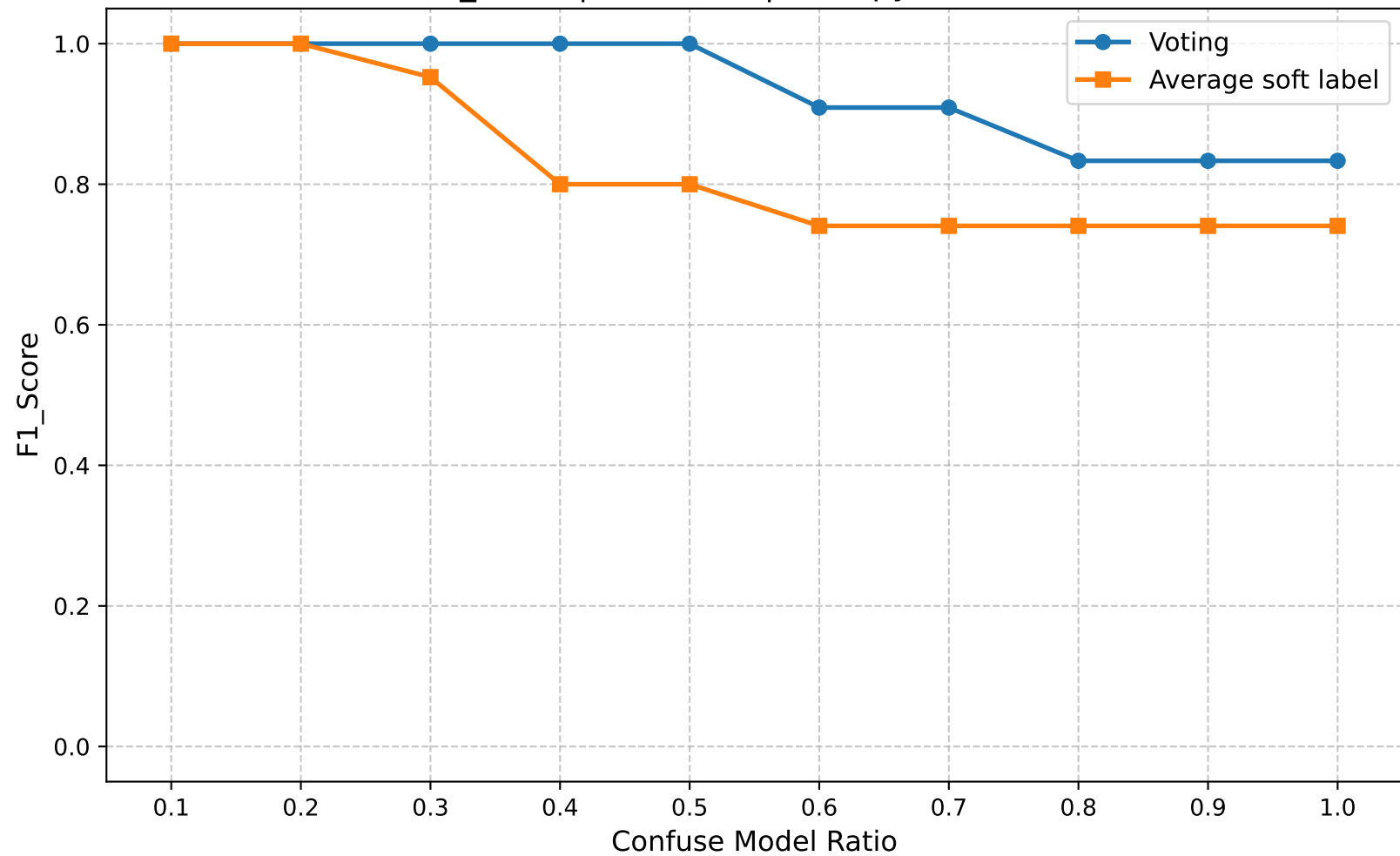
F1_Score | Round 20 | Entropy Ratio 0.80
