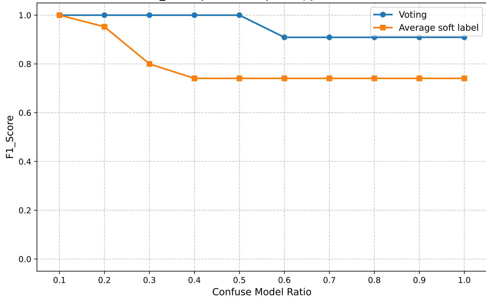
F1_Score | Round 20 | Entropy Ratio 0.85
