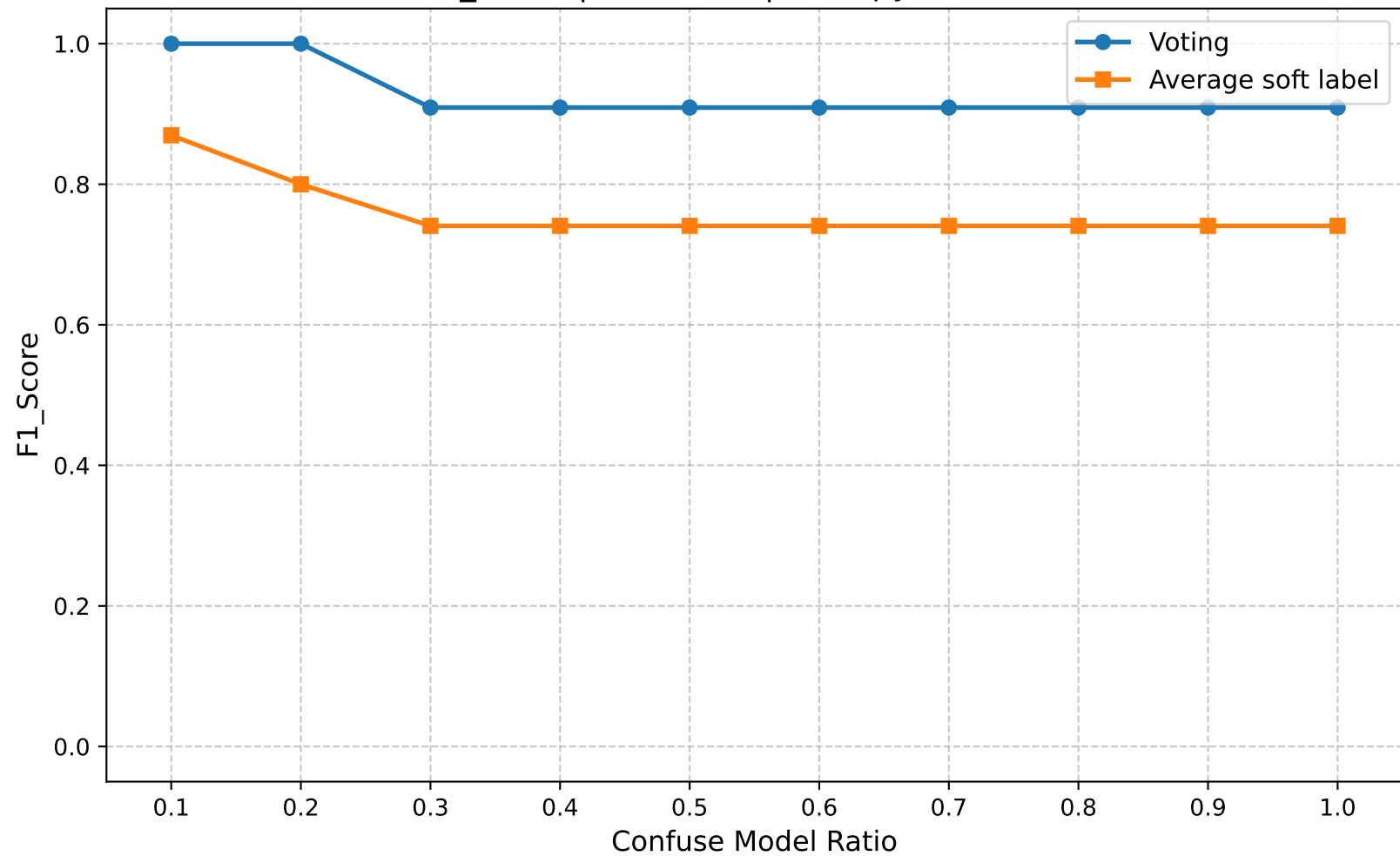
F1_Score | Round 20 | Entropy Ratio 0.95
