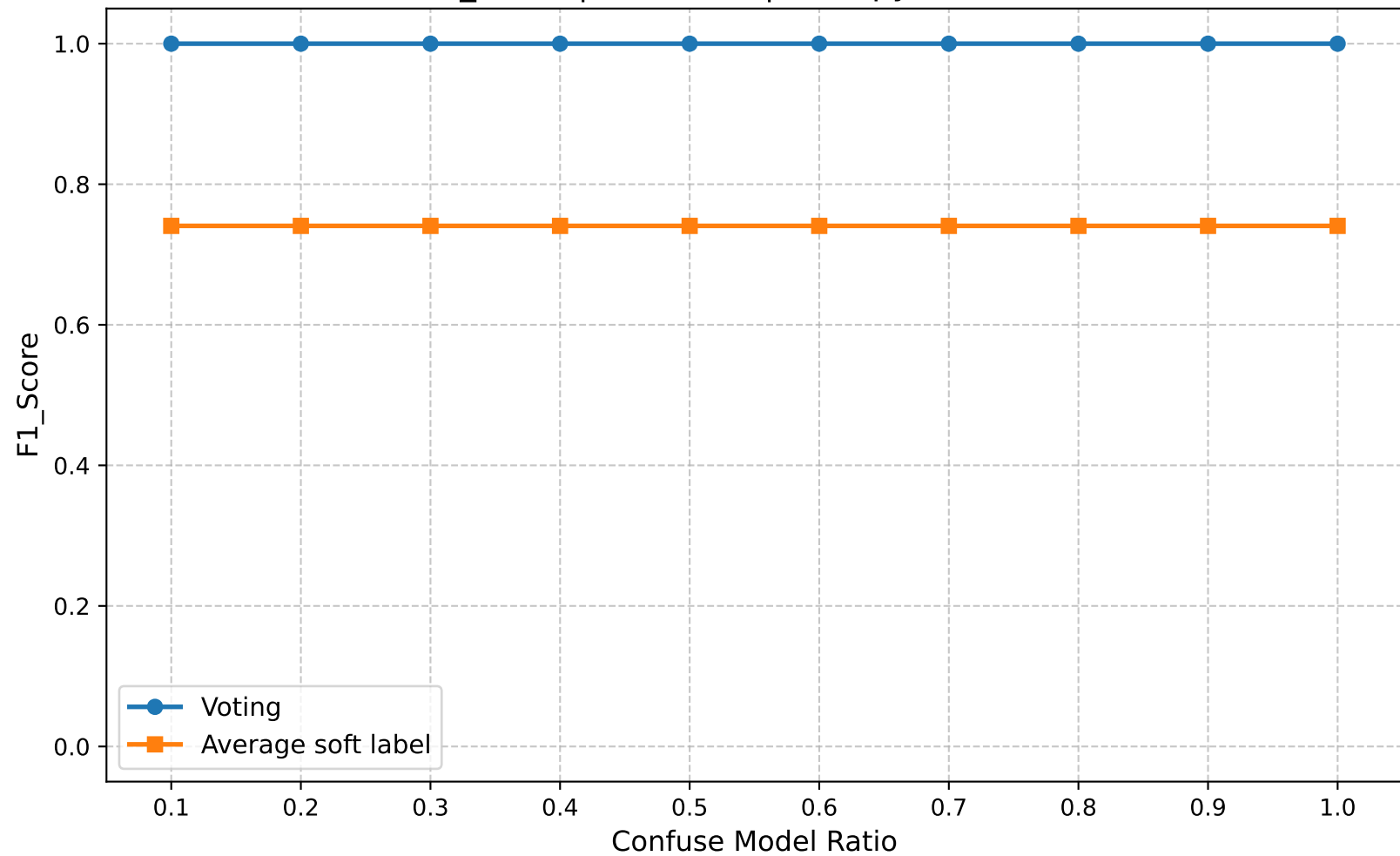
F1_Score | Round 20 | Entropy Ratio 1.00
