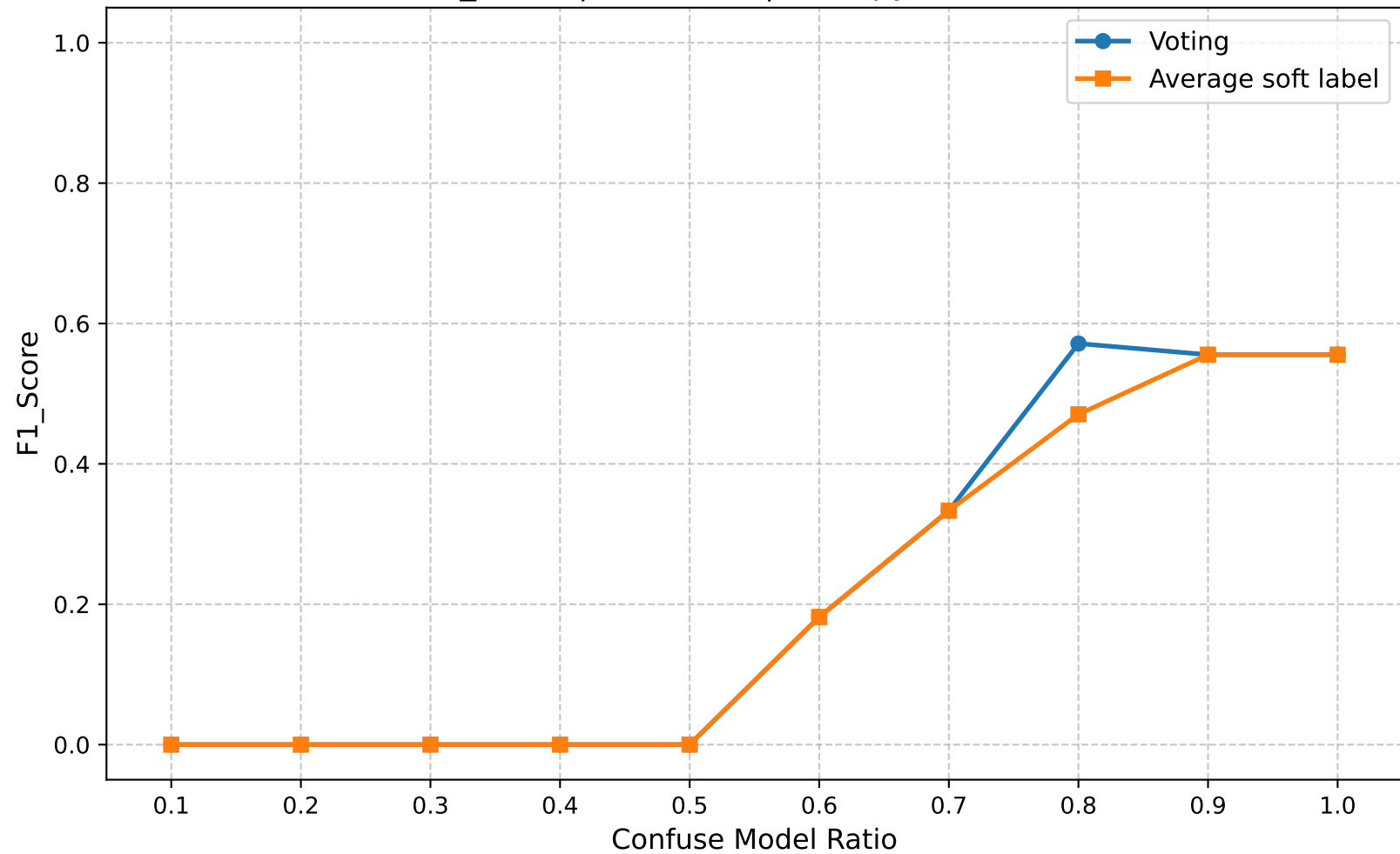
F1_Score | Round 25 | Entropy Ratio 0.10
