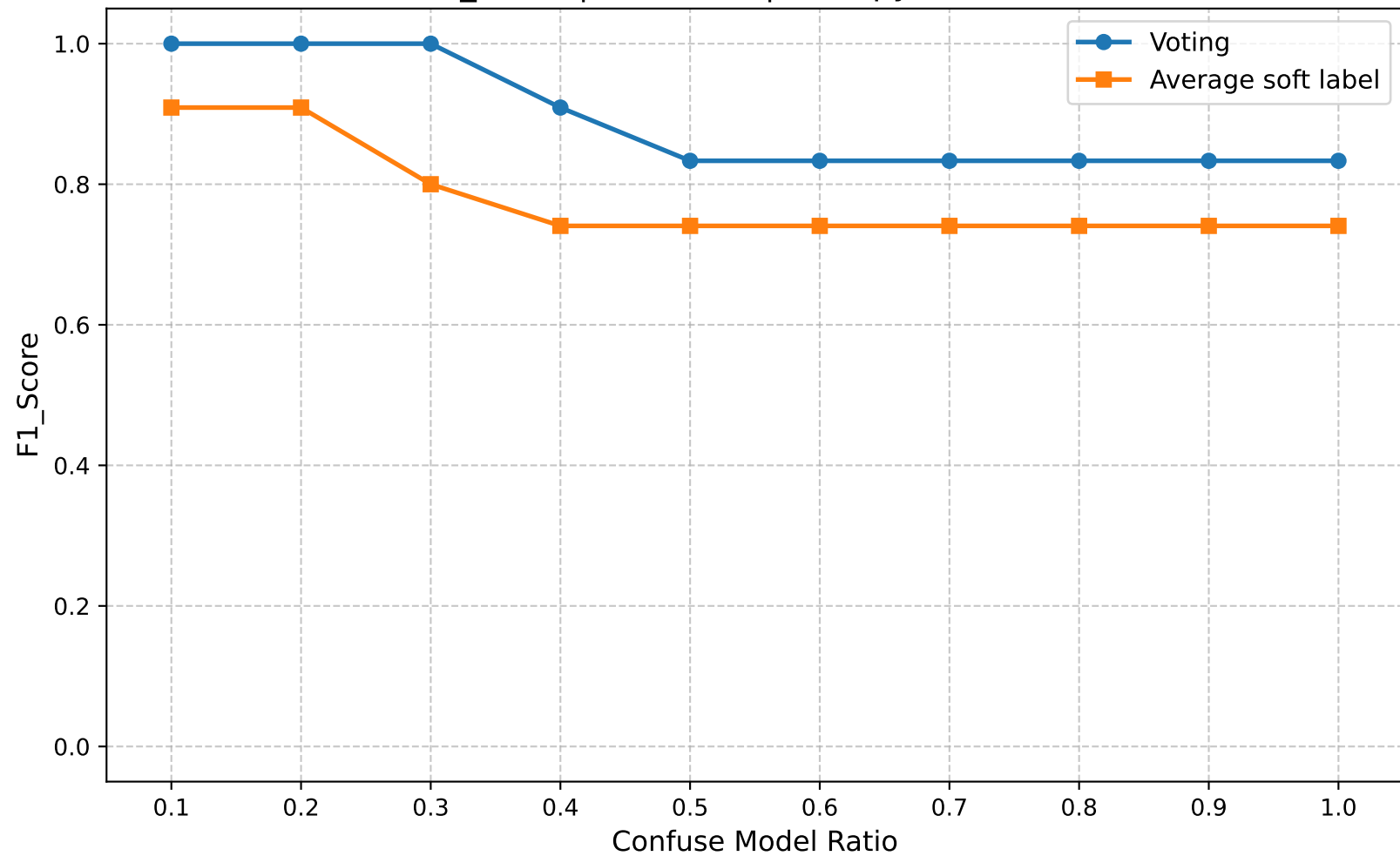
F1_Score | Round 25 | Entropy Ratio 0.90
