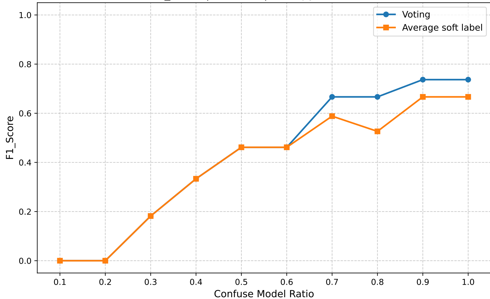
F1_Score | Round 5 | Entropy Ratio 0.15
