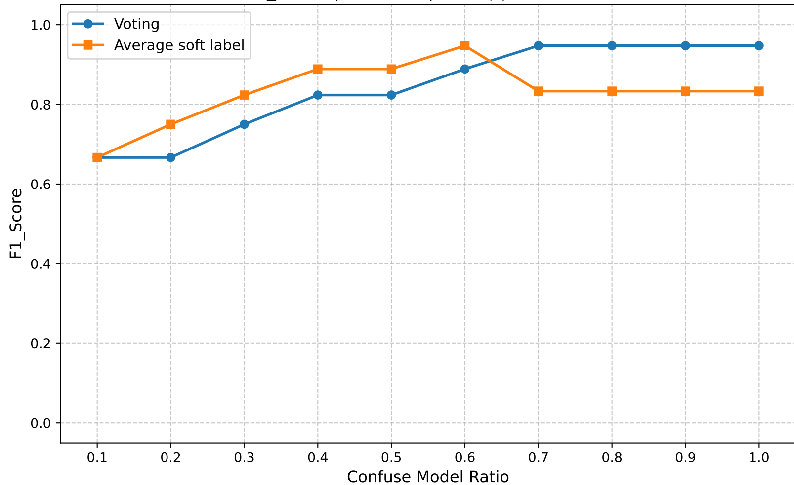
F1_Score | Round 5 | Entropy Ratio 0.40
