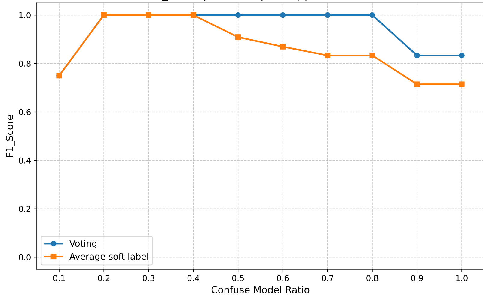
F1_Score | Round 5 | Entropy Ratio 0.55
