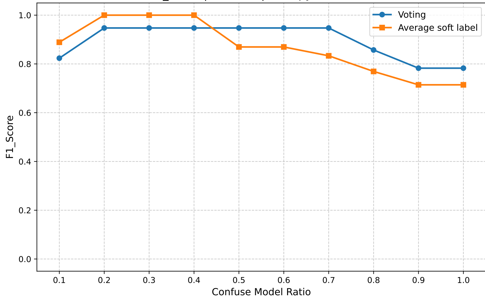
F1_Score | Round 5 | Entropy Ratio 0.60
