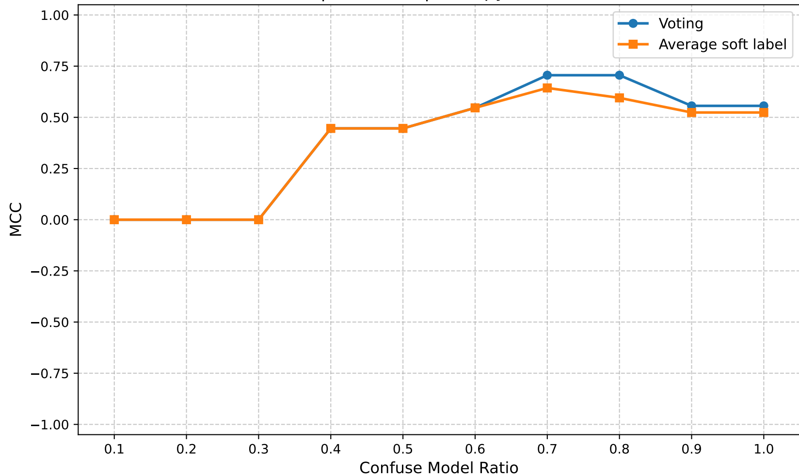
MCC | Round 10 | Entropy Ratio 0.15
