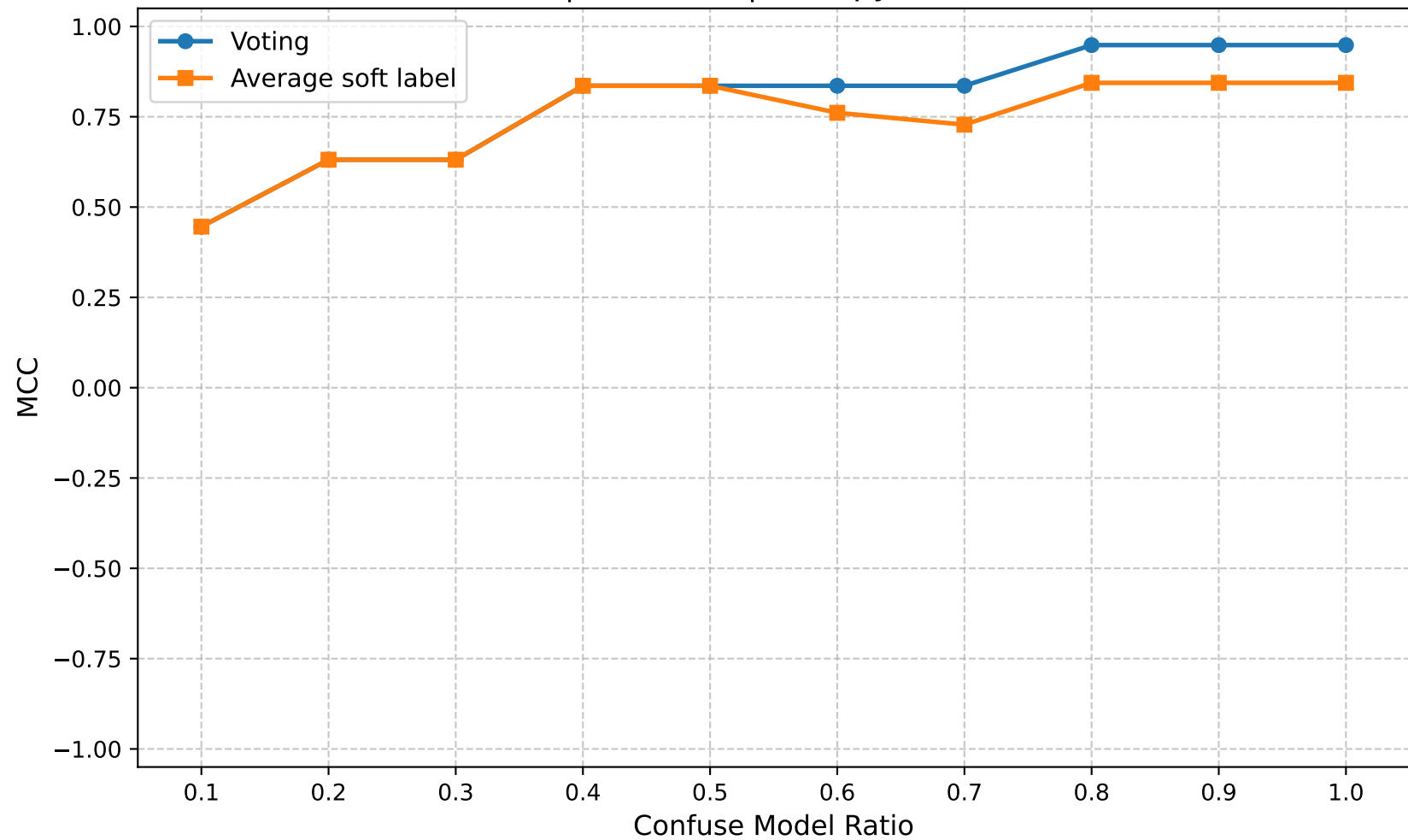
MCC | Round 10 | Entropy Ratio 0.35
