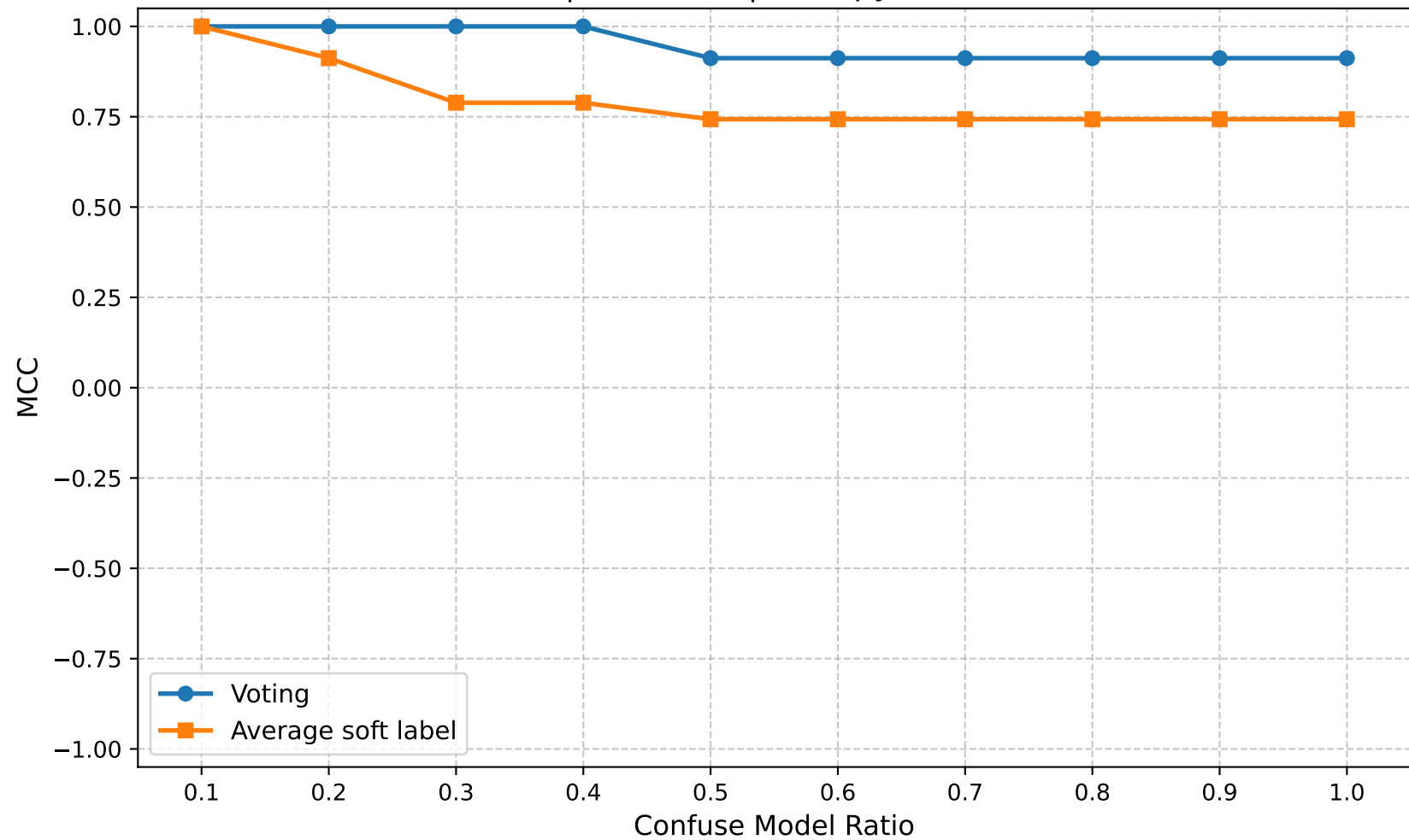
MCC | Round 10 | Entropy Ratio 0.85
