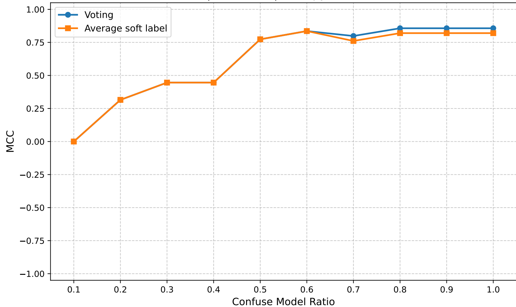
MCC | Round 15 | Entropy Ratio 0.30
