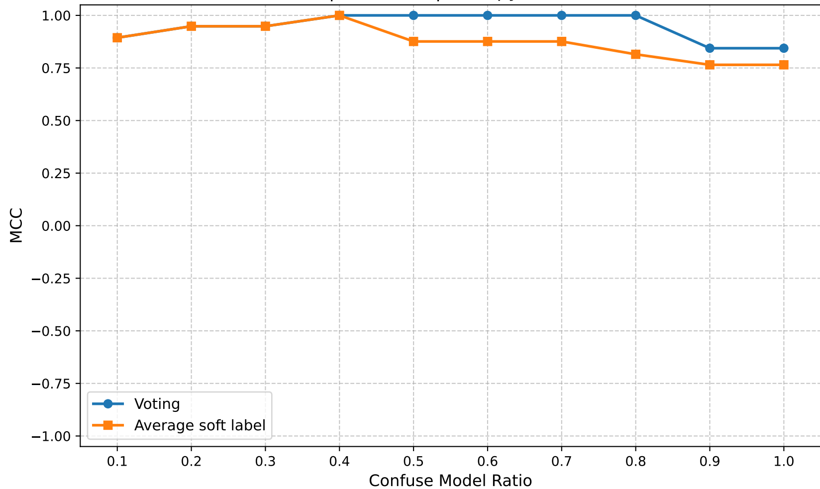
MCC | Round 15 | Entropy Ratio 0.60
