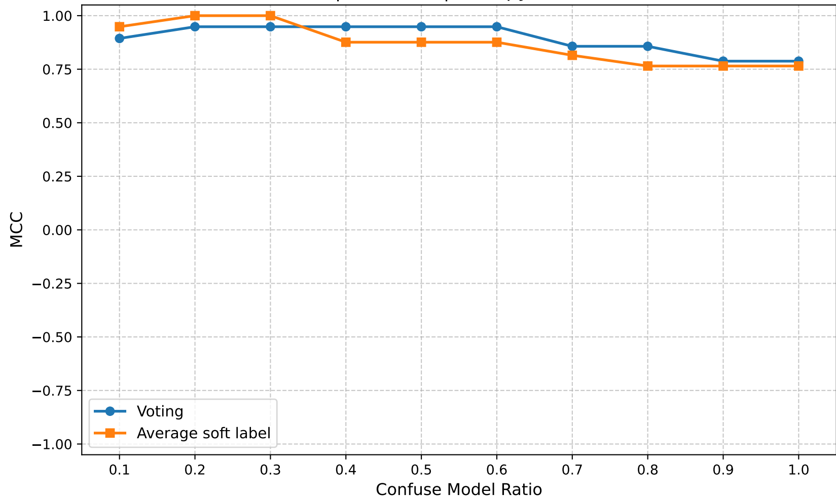
MCC | Round 15 | Entropy Ratio 0.70
