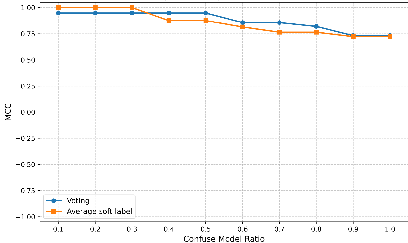
MCC | Round 15 | Entropy Ratio 0.75
