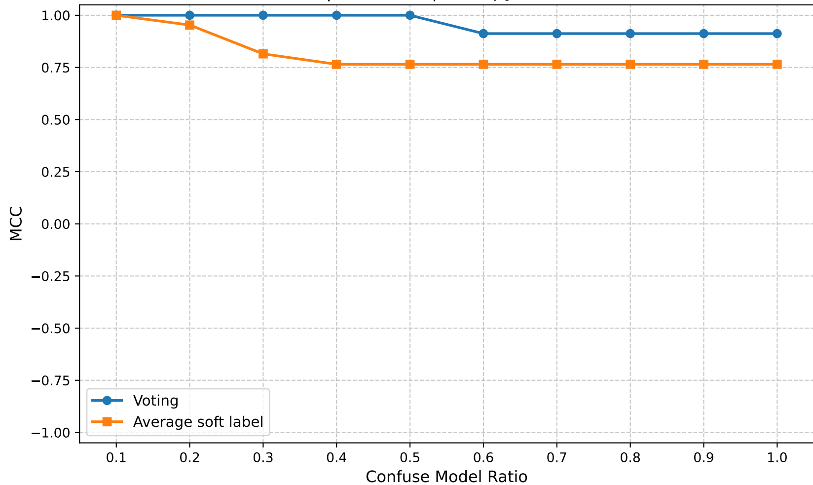
MCC | Round 20 | Entropy Ratio 0.85
