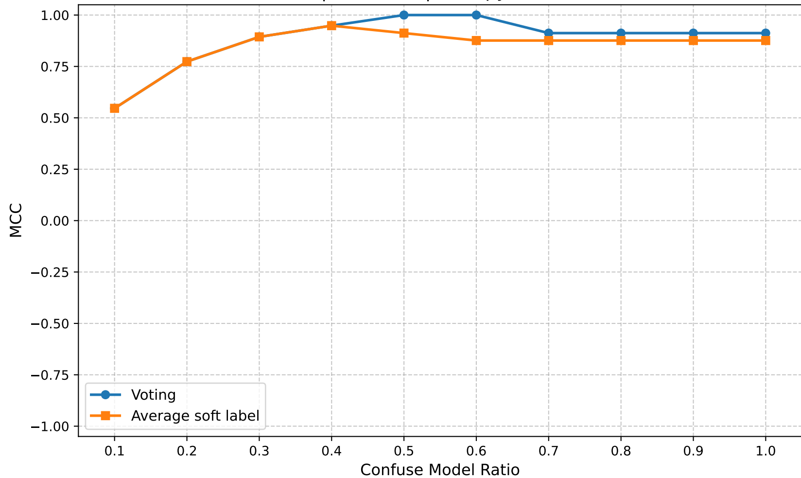
MCC | Round 25 | Entropy Ratio 0.45
