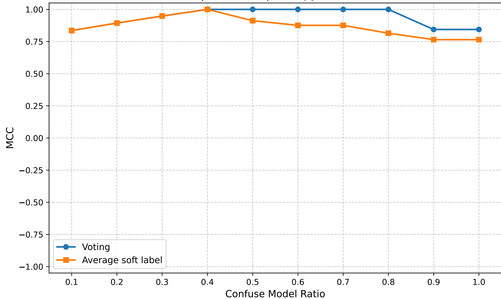
MCC | Round 25 | Entropy Ratio 0.60
