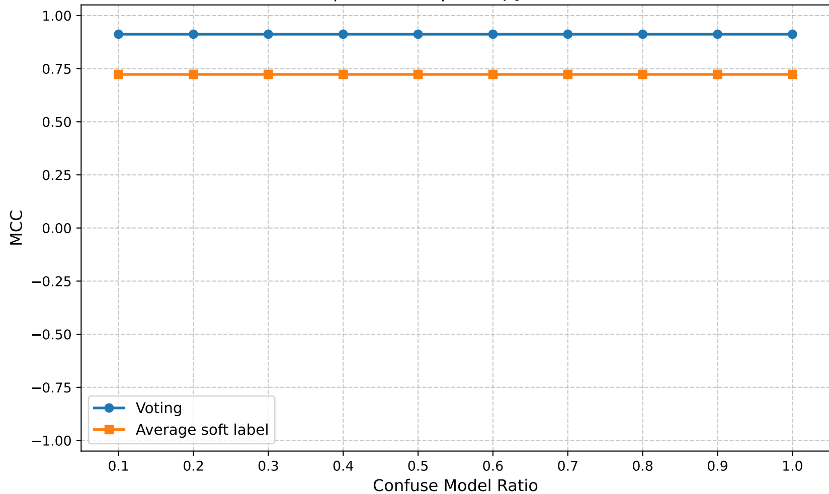
MCC | Round 25 | Entropy Ratio 1.00
