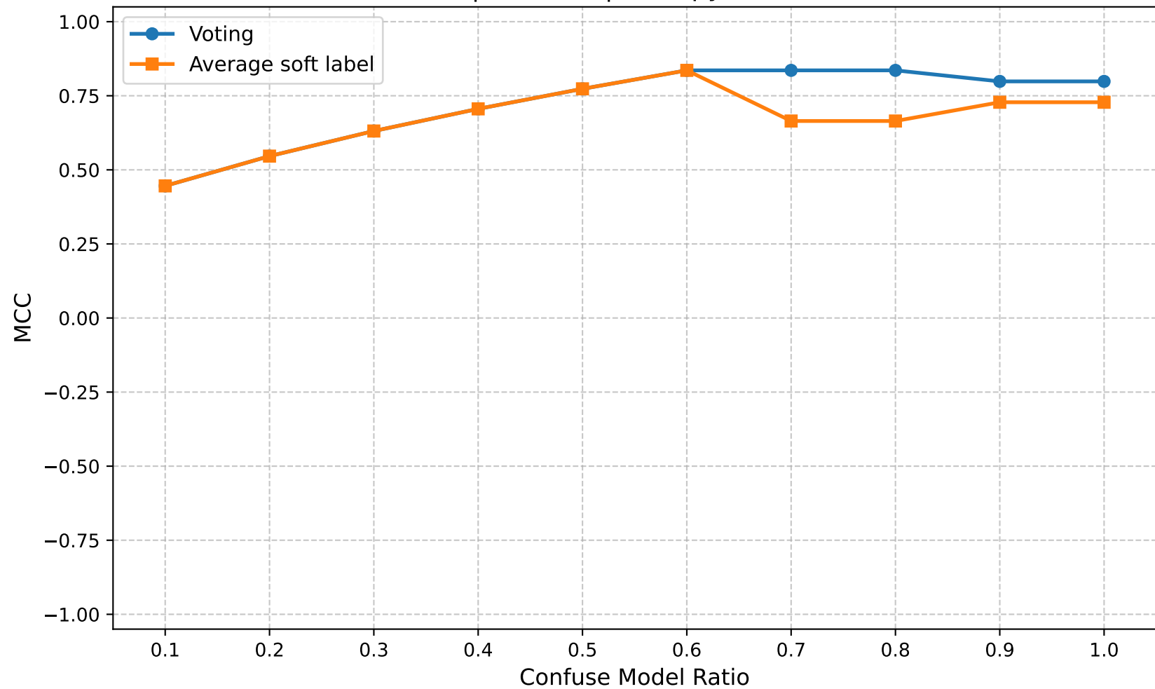
MCC | Round 5 | Entropy Ratio 0.25
