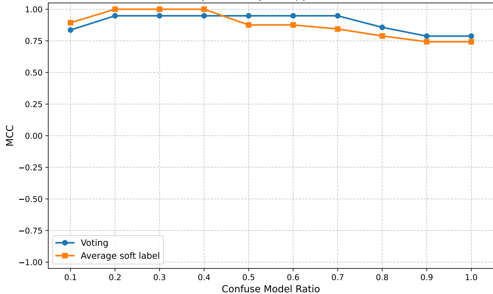
MCC | Round 5 | Entropy Ratio 0.60
