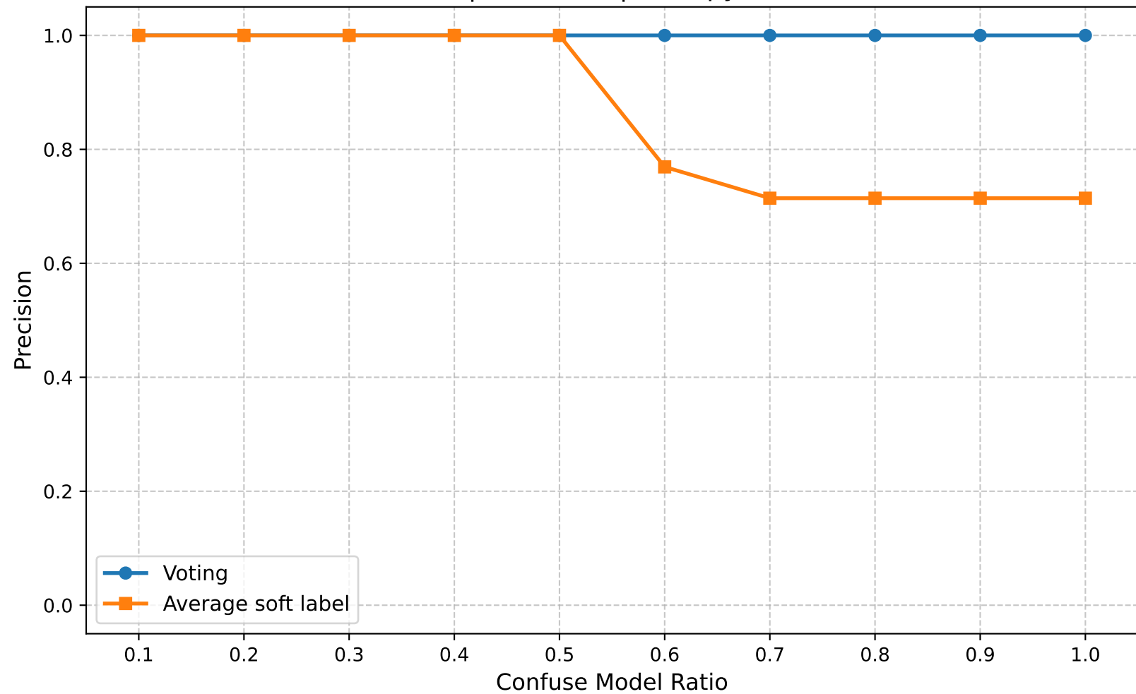
Precision | Round 10 | Entropy Ratio 0.45
