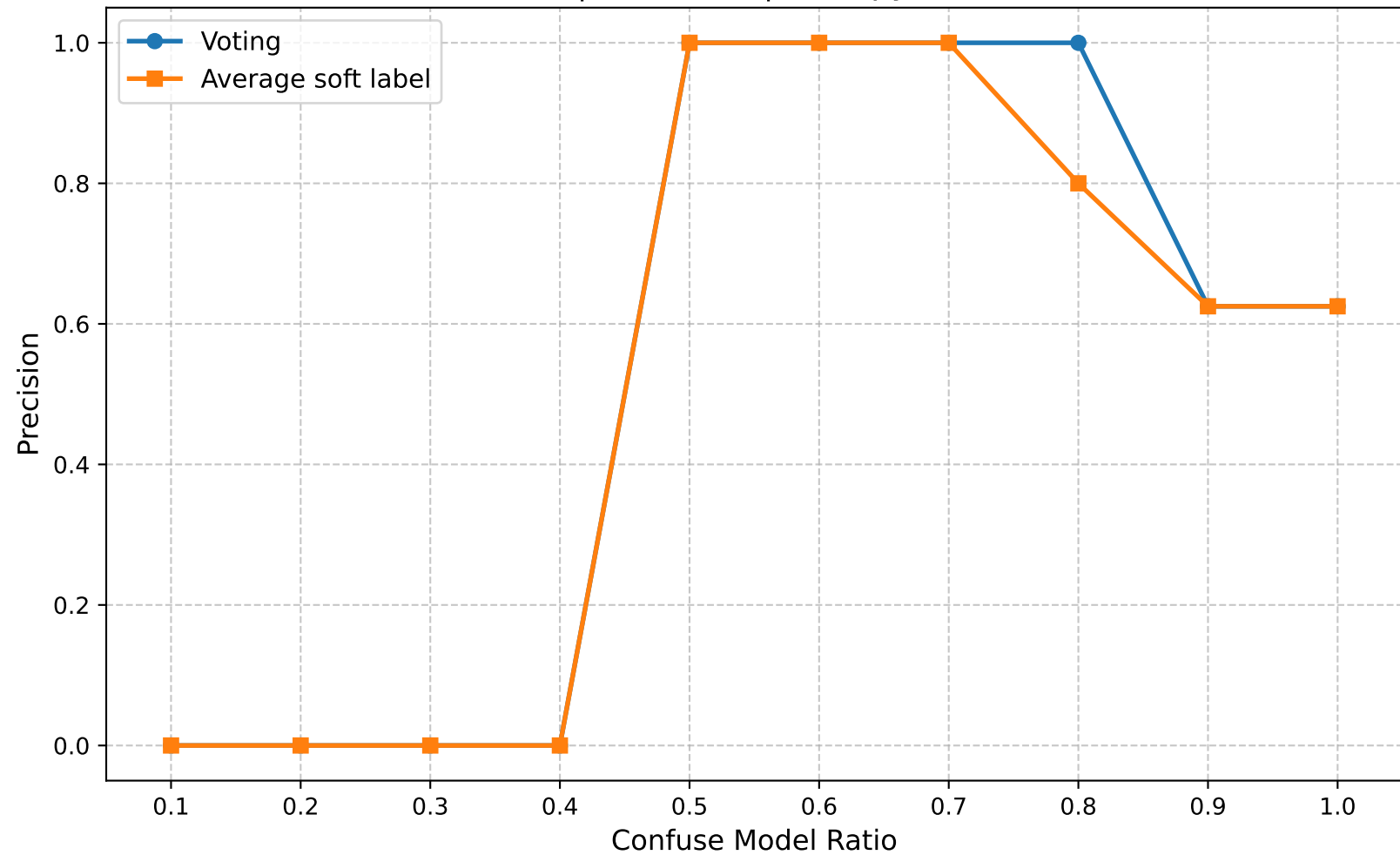
Precision | Round 15 | Entropy Ratio 0.15
