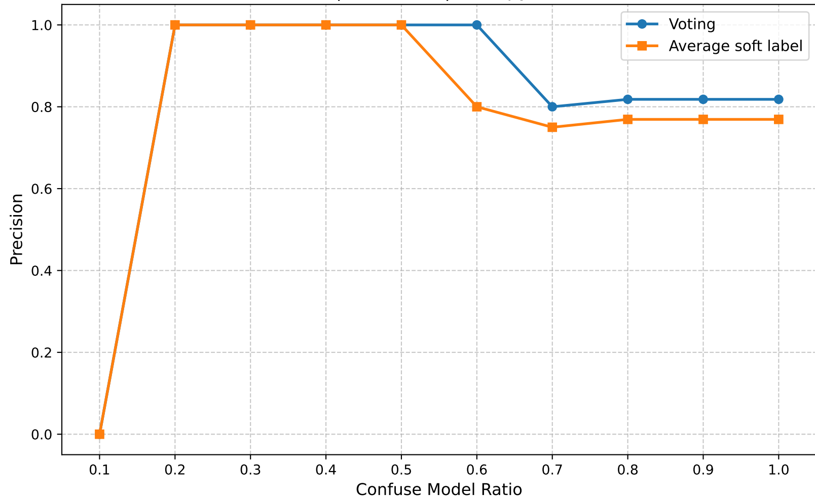
Precision | Round 15 | Entropy Ratio 0.35
