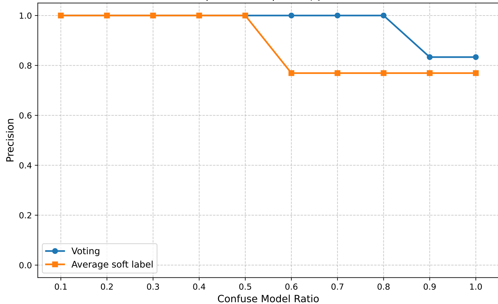
Precision | Round 15 | Entropy Ratio 0.50
