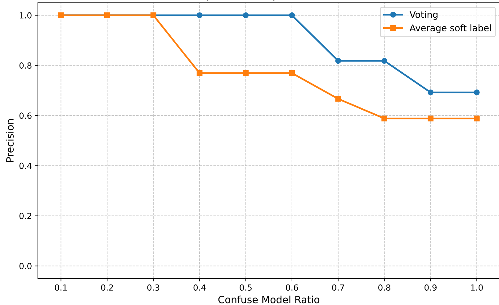
Precision | Round 15 | Entropy Ratio 0.70
