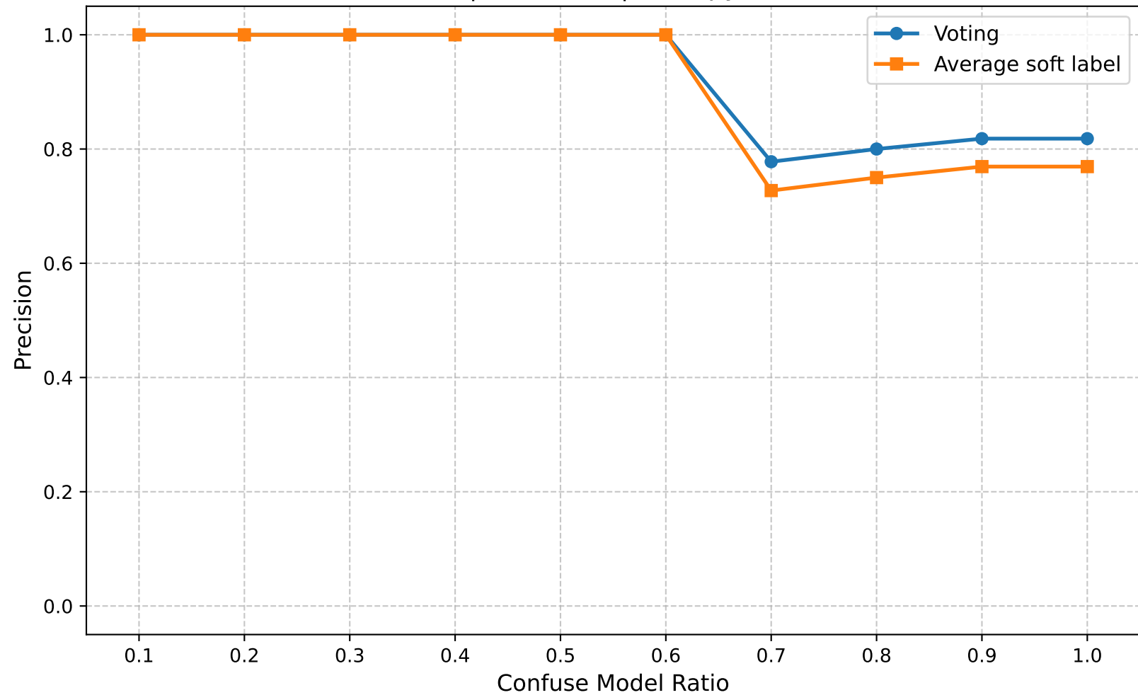
Precision | Round 25 | Entropy Ratio 0.30
