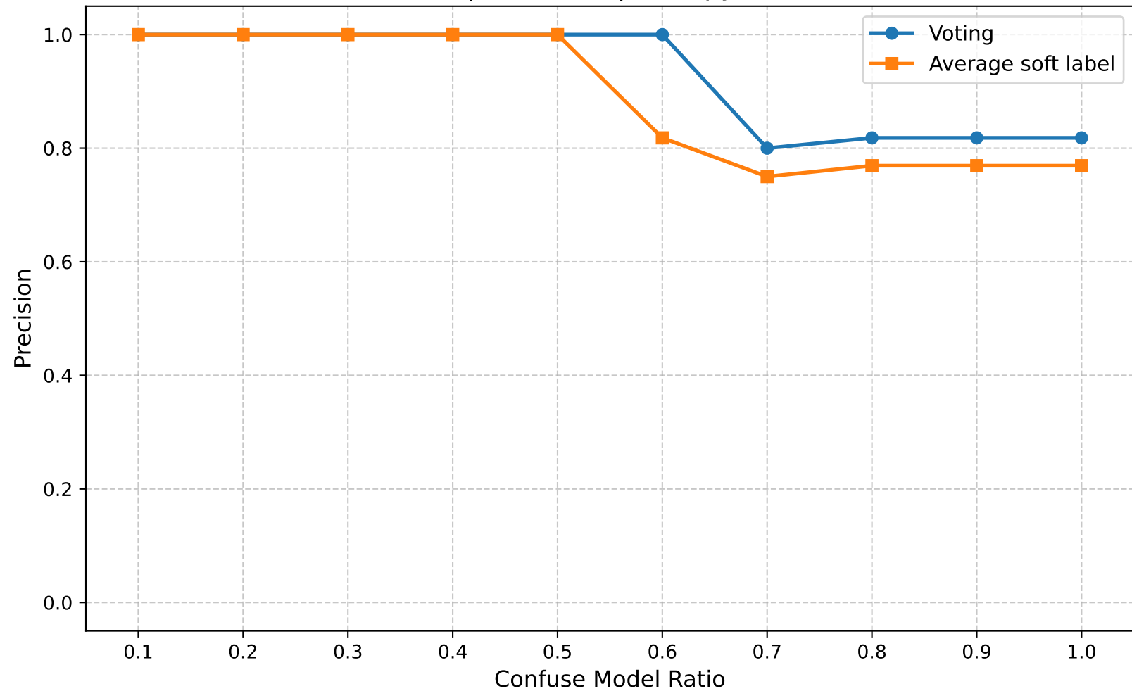
Precision | Round 25 | Entropy Ratio 0.35
