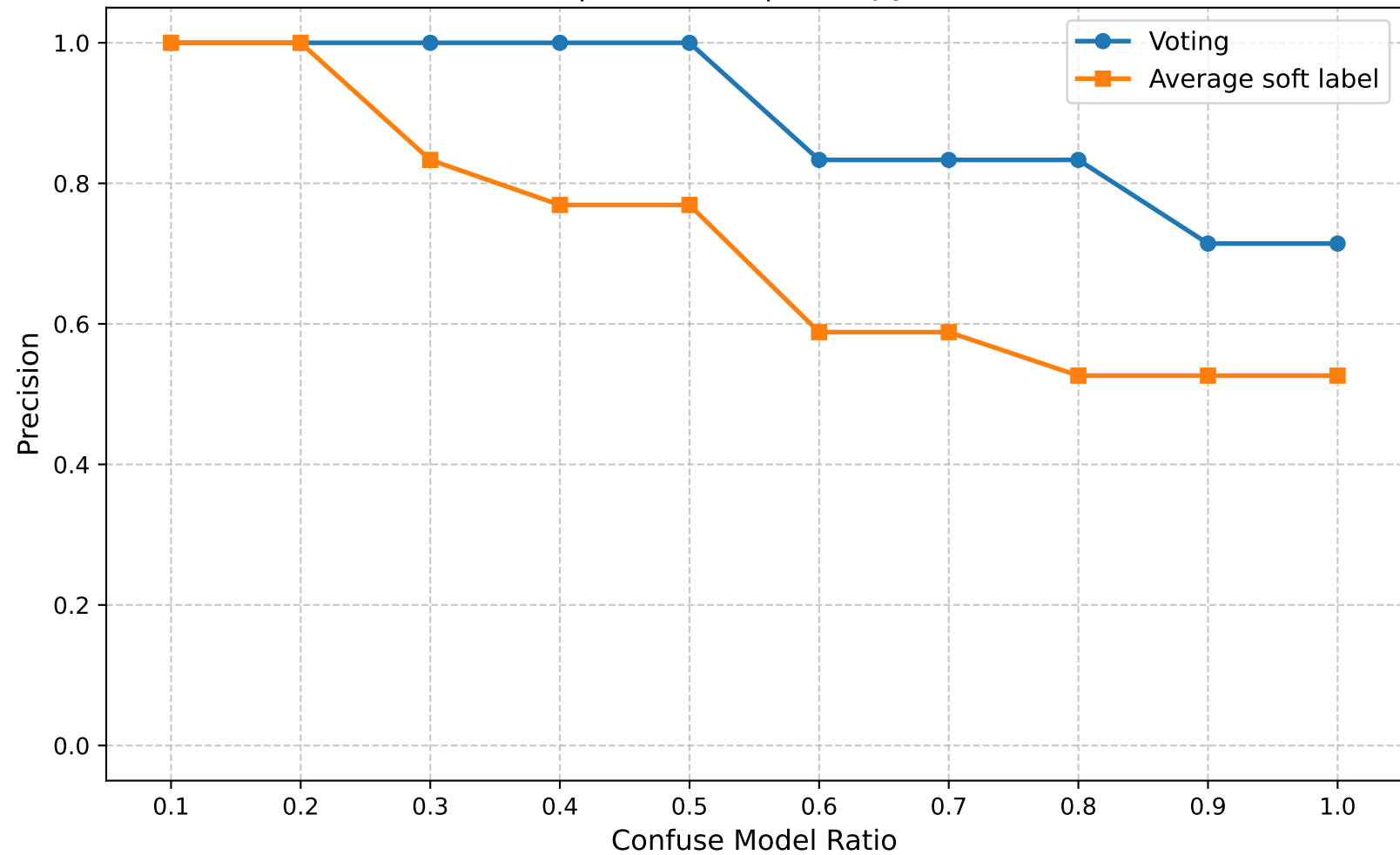
Precision | Round 25 | Entropy Ratio 0.75
