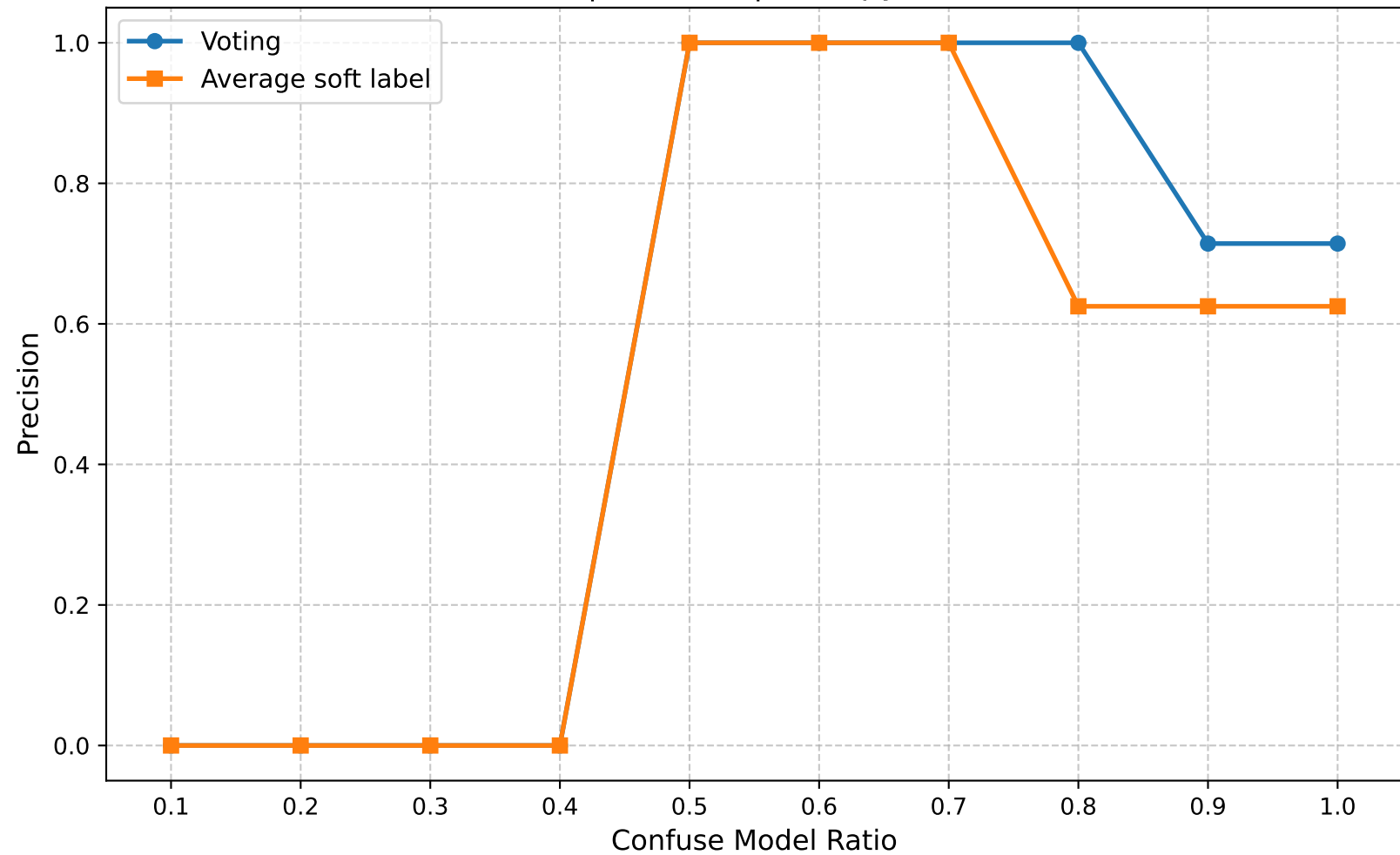
Precision | Round 5 | Entropy Ratio 0.10
