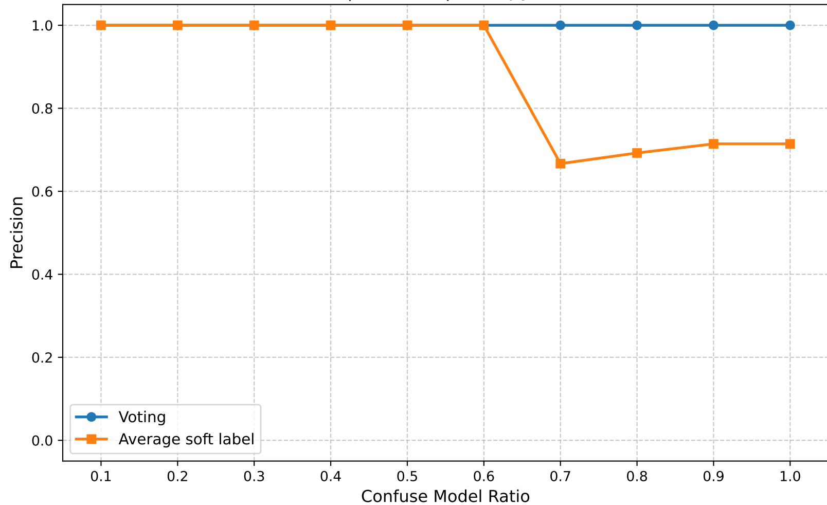
Precision | Round 5 | Entropy Ratio 0.30
