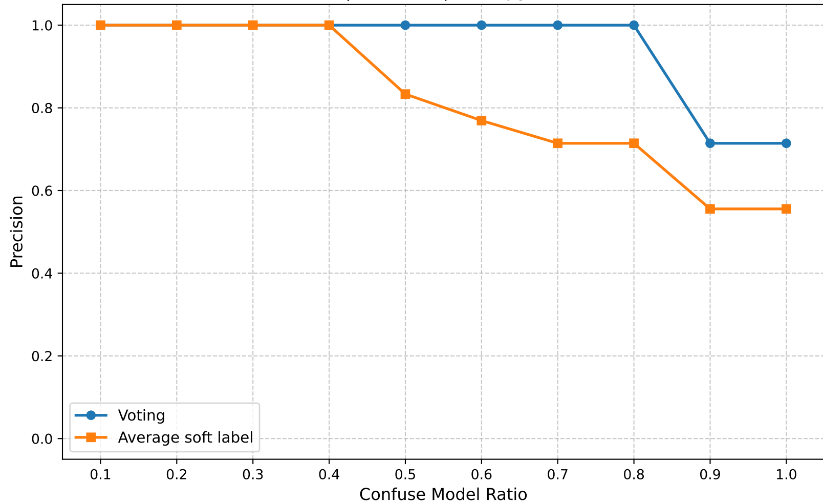
Precision | Round 5 | Entropy Ratio 0.55
