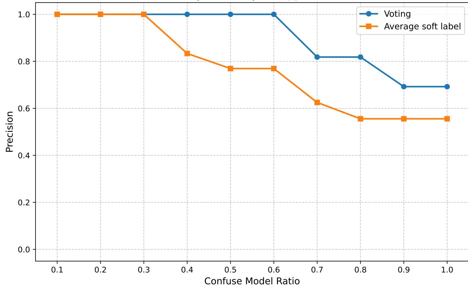
Precision | Round 5 | Entropy Ratio 0.65
