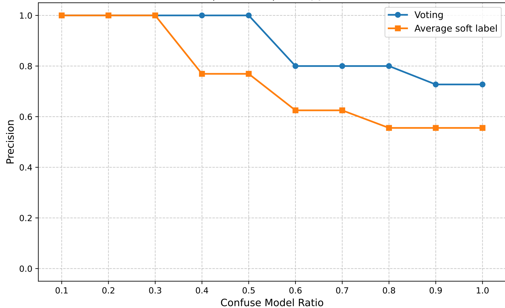
Precision | Round 5 | Entropy Ratio 0.70
