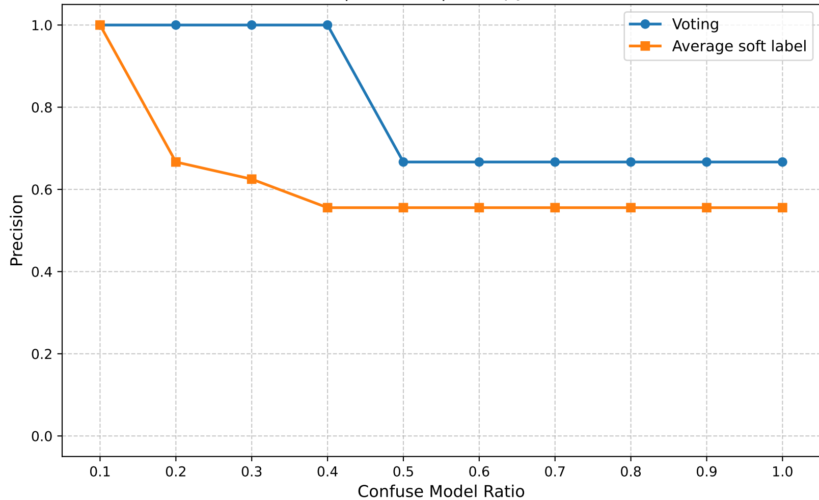
Precision | Round 5 | Entropy Ratio 0.90
